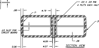
SECTION VIEW
